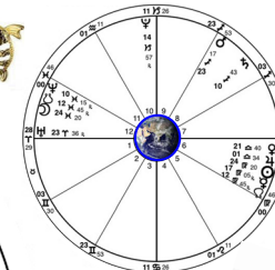
2016 Pisces Lunar Eclipse September 16, 2016 19:05:04 UT
