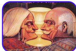
Sabian Symbol 9/1/16 Virgo New Moon: Two heads looking out & beyond shadows Salvador Dali "Old Couple or Musician"
