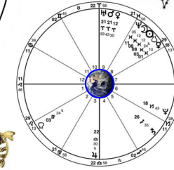
2017 Pisces Solar Eclipse February 26, 2017 14:58:24 UT
