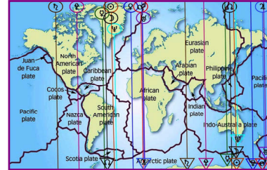
2/26/17 Premier Solar Eclipse Tectonic Cosmology AMP Cartography Composite
