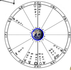
2017 Leo Lunar Eclipse February 11, 2017 00:33:33 UT
