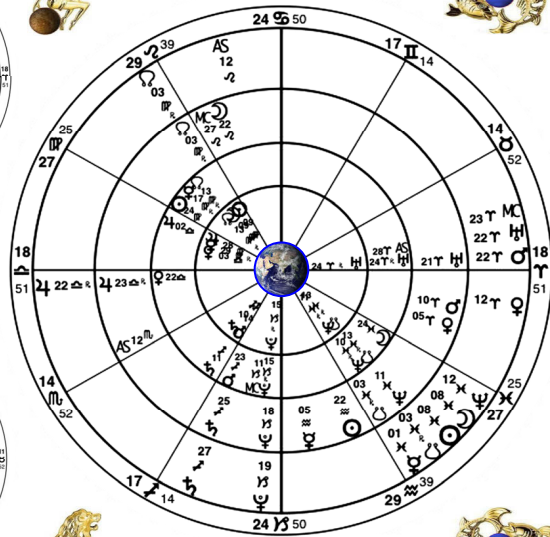
Our Late 2016 & Early 2017 Eclipses Astral Metaphysics Publishing™
