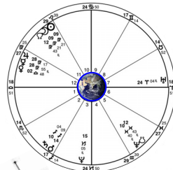
2016 Virgo Solar Eclipse September 1, 2016 09:03:16 UT
